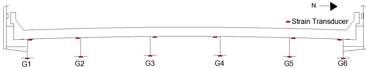
Figure 9. Sioux County Bridge cross-section view of strain transducer locations
